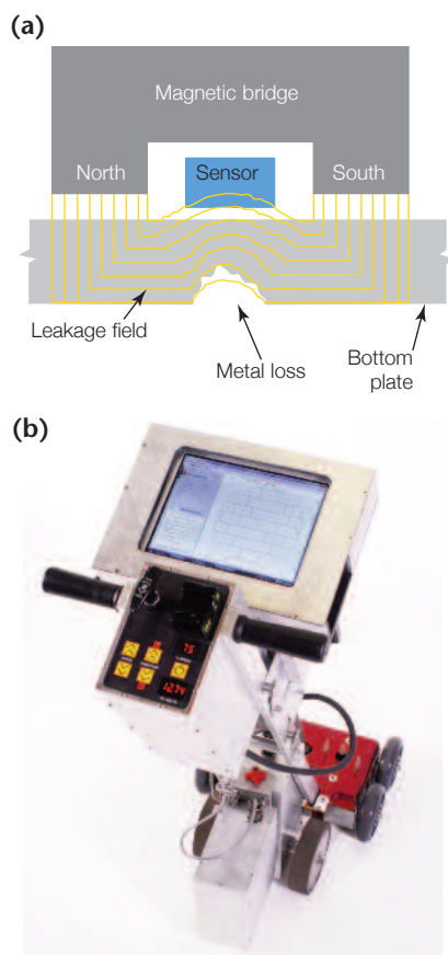
Figure 2. Magnetic flux leakage method: (a) schematic of bridge; (b) tank bottom scanner incorporating magnetic flux leakage test bridge.
